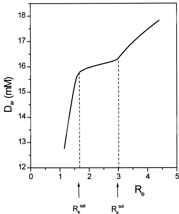
Fig. 4. An approximate dependence of the concentration of detergent monomers ( D_w ) in mixtures of PC and the non-ionic detergent OG on the OG/PC ratio in mixed aggregates ( R_e ). The dependence is based on isothermal calorimetric titration of OG/PC mixed micelles according to protocol I (Fig. 1), as interpreted [18] under the assumption that the main contribution to \Delta Q is due to extraction of OG monomers from OG/PC mixed aggregates (with constant \Delta H_D^{\text{a} \rightarrow \text{w}} ).
