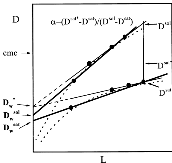
Fig. 3. Illustration of the phase boundaries in lipid-detergent mixed dispersions. The detergent concentrations required for the onset ( D^{\text{sat}} ) and completion ( D^{\text{sol}} ) are plotted as functions of the lipid concentration. Note that the bold lines intersect the detergent axis (at D_w^{\text{sat}} and D_w^{\text{sol}} ) below D_w^* , which is the common concentration of monomers in aqueous solutions at high absolute concentrations of lipid and detergent. The broken lines illustrate the expected non-linear dependence (see text for details).
